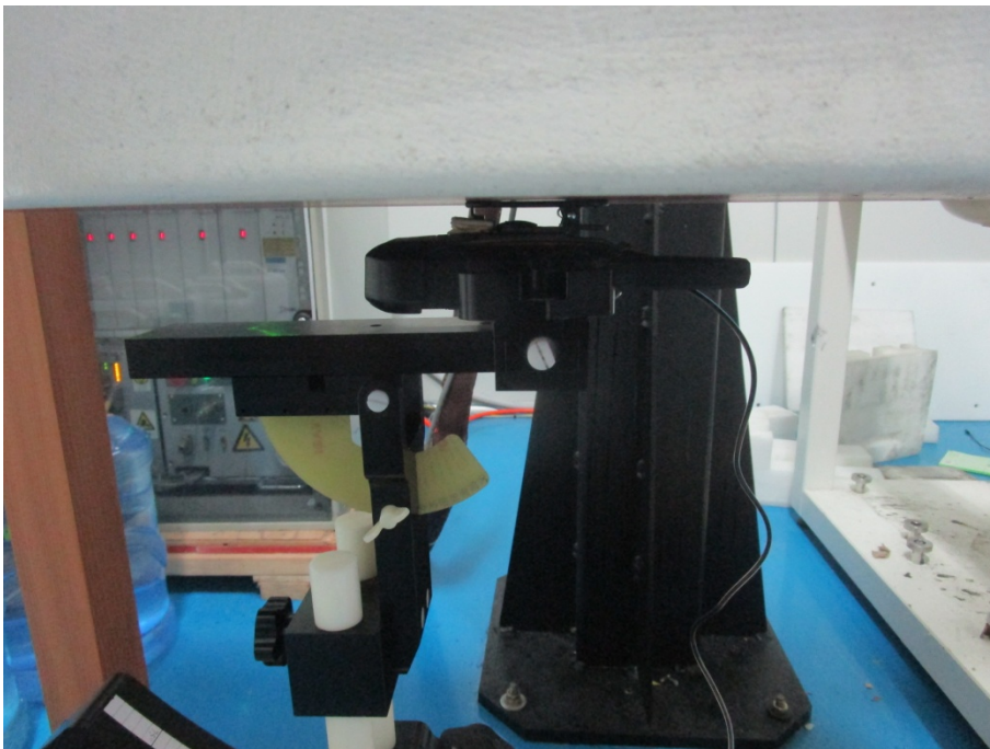
Body Back with Headset 2 Setup Photo (0mm)
