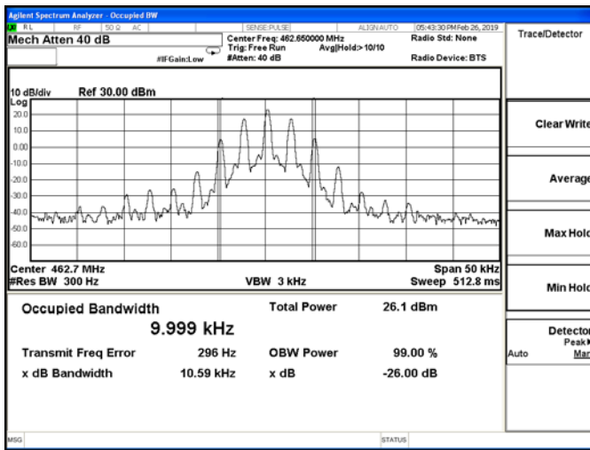
Channel 19: 462.6500MHz
