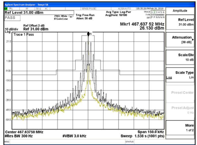
Channel 11: 467.6375MHz
