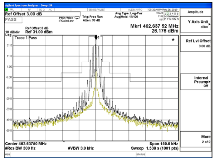
Channel 4: 462.6375MHz
