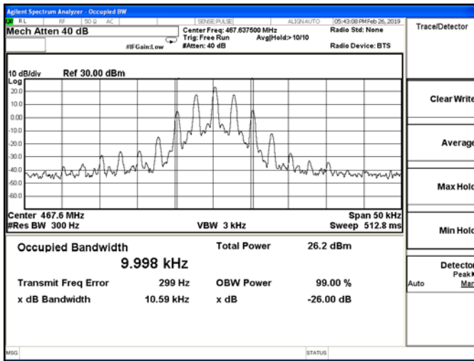
Channel 11: 467.6375MHz
