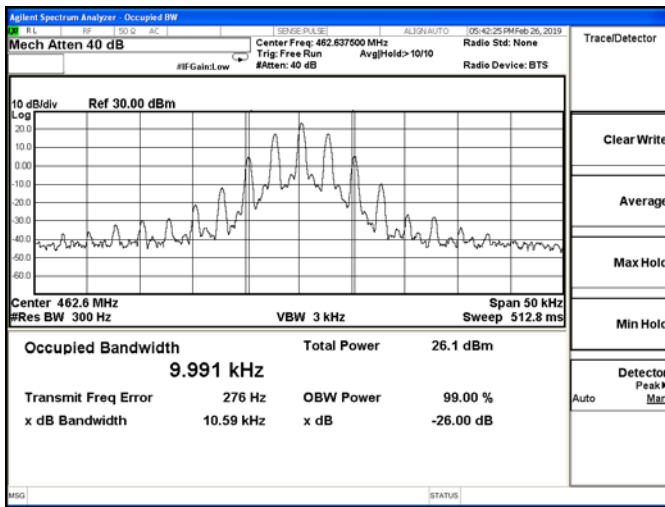
Channel 4: 462.6375MHz
