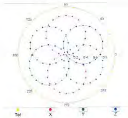
f=600 MHz,TEM
