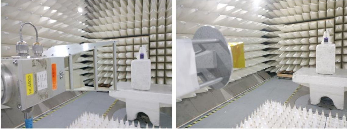
Photograph No.4 Spurious and band edge emissions measurement setup in the anechoic chamber above 1 GHz
