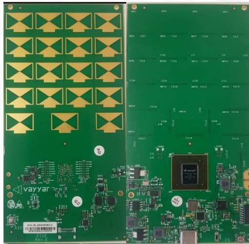
Figure 1: VMAKERPROUWB module utilizing USB interface for communication with hosting device
