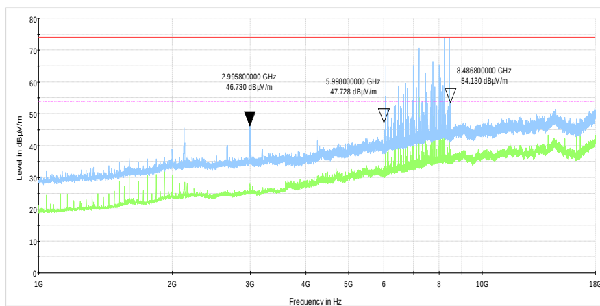
Plot 7.3.4 Radiated emission measurements in 1 – 18 GHz range according to the Section 15.209
