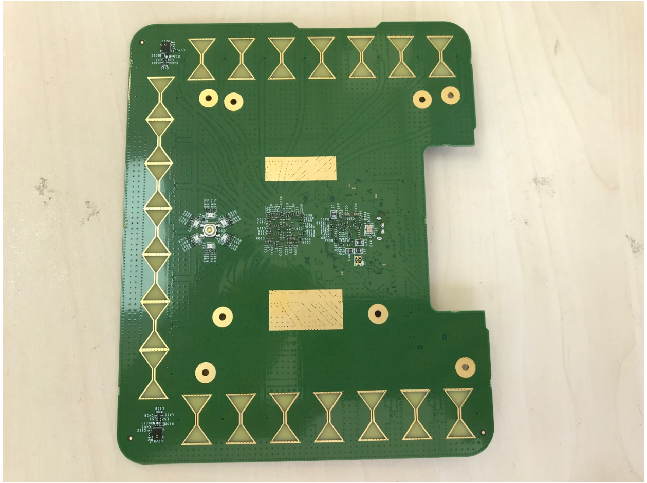
Figure 2: Rear View
