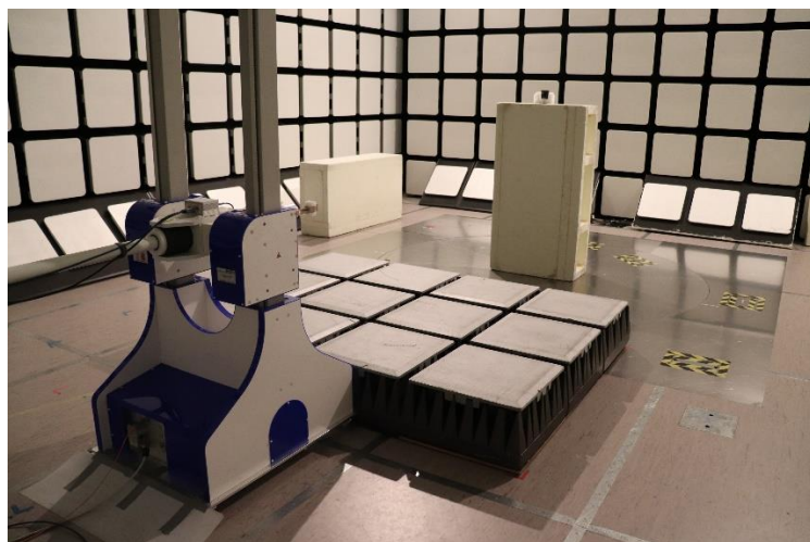
Photograph 6. Radiated Emissions 18 – 26.5 GHz
