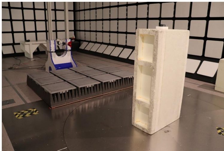
Photograph 5. Radiated Emissions 1 – 18 GHz
