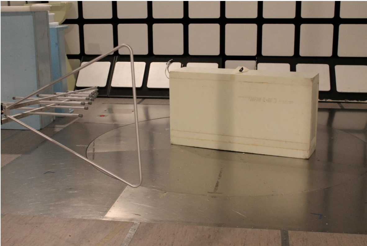
Photograph 4. Radiated emission setup below 1 GHz.
