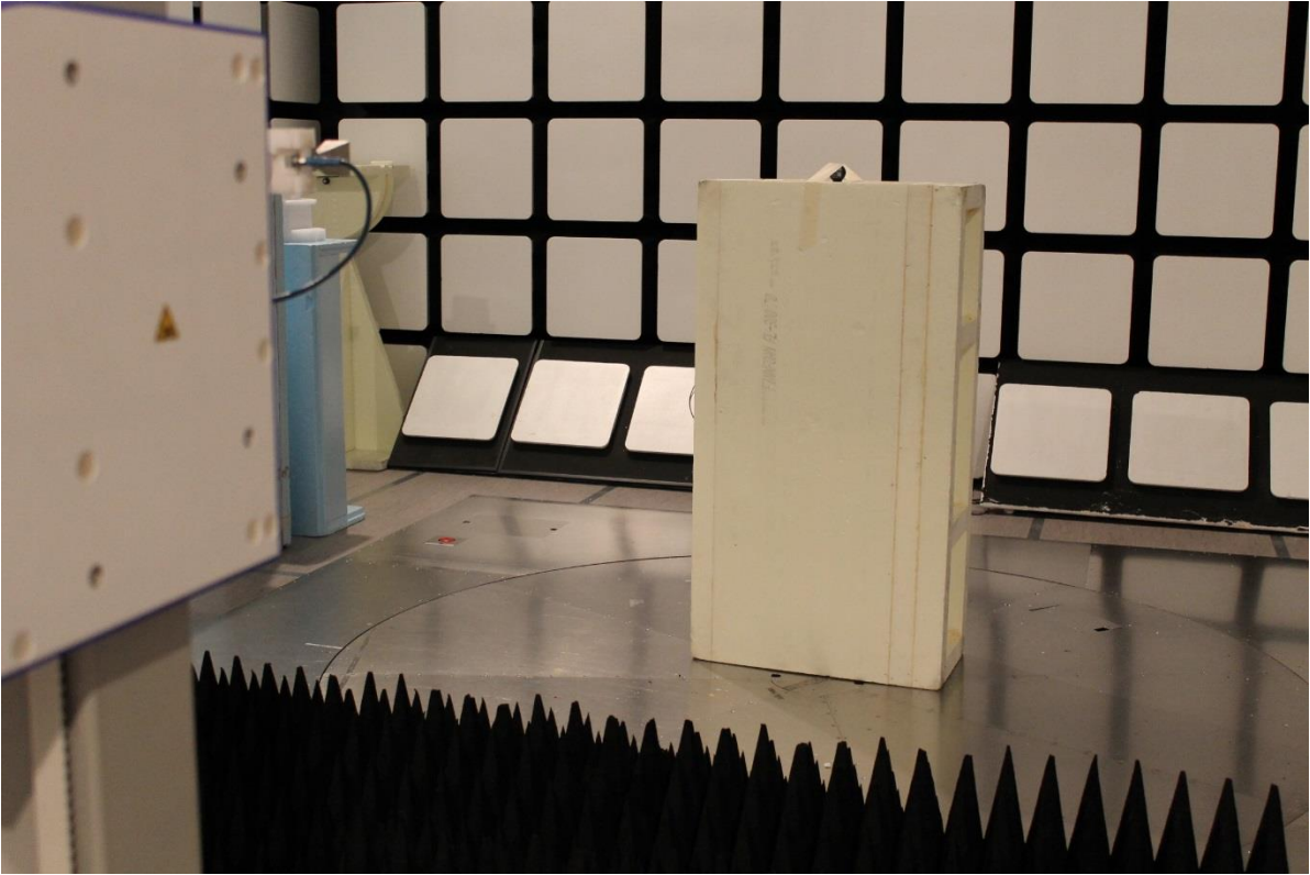
Photograph 5. Radiated emission setup above 1 GHz.
