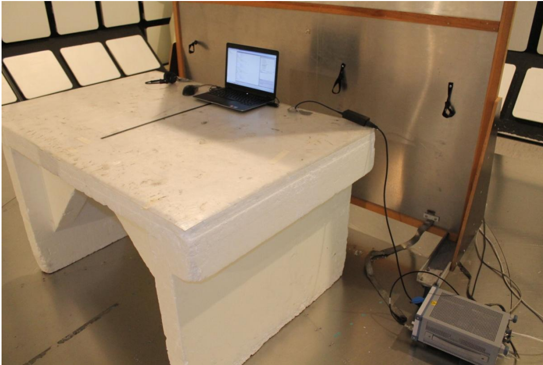
Photograph 3. Conducted emission setup.
