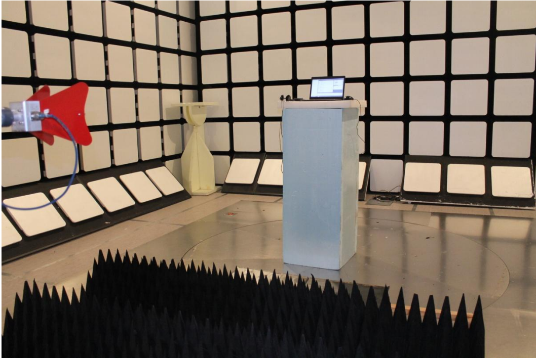
Photograph 3. Radiated emission 1 GHz to 18 GHz.
