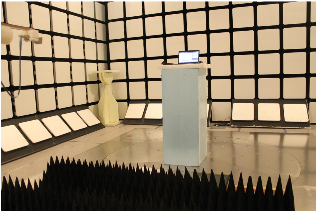
Photograph 4. Radiated emission 18 to 26 GHz.
