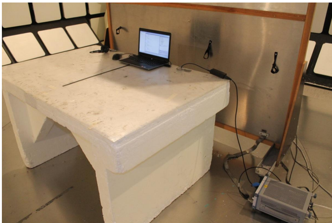
Photograph 5. Conducted emission setup.
