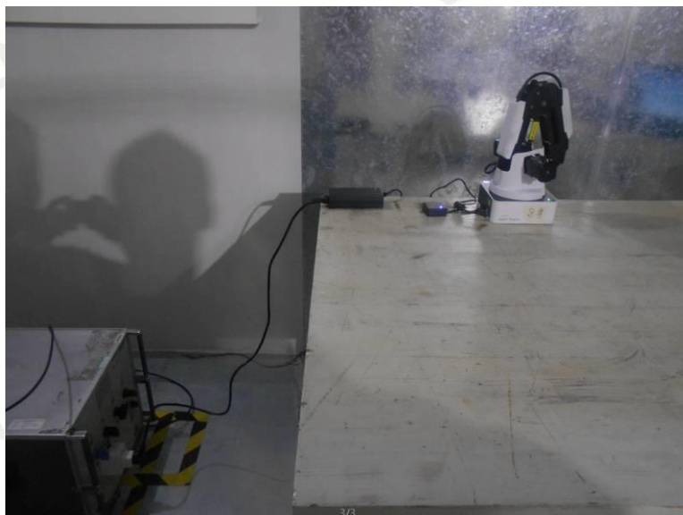
Conducted emission
