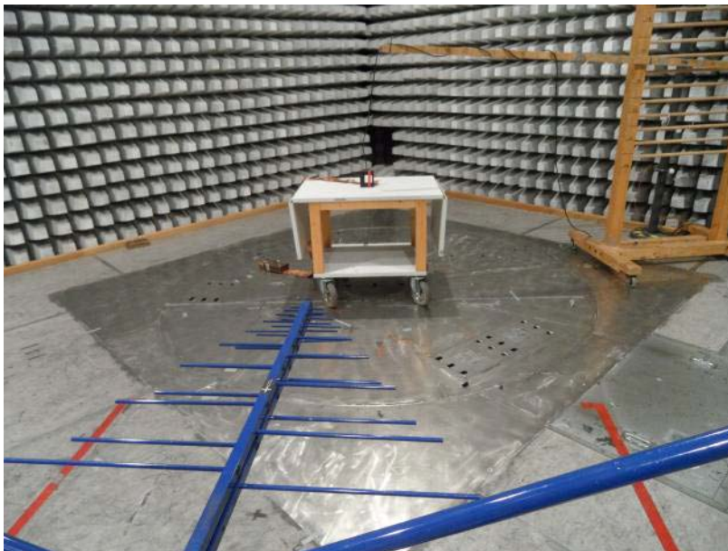
Figure 2: test setup for Radiated disturbances 30 MHz to 1000 MHz
