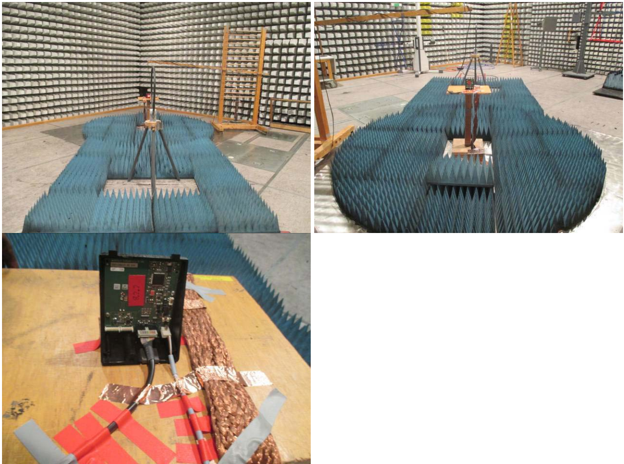
Figure 3: test setup for Radiated disturbances 9 kHz to 30 MHz
