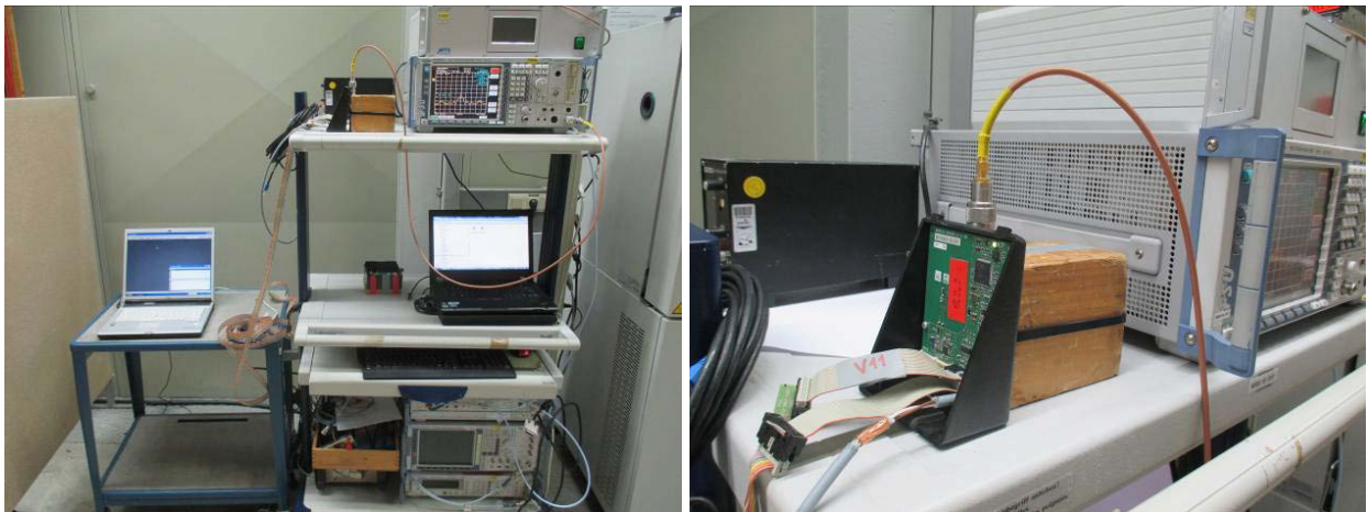
Figure 1: Test Setup Occupied Bandwidth
