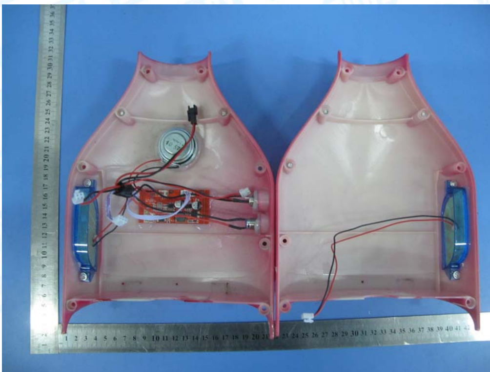
Photo 8 Internal of EUT
