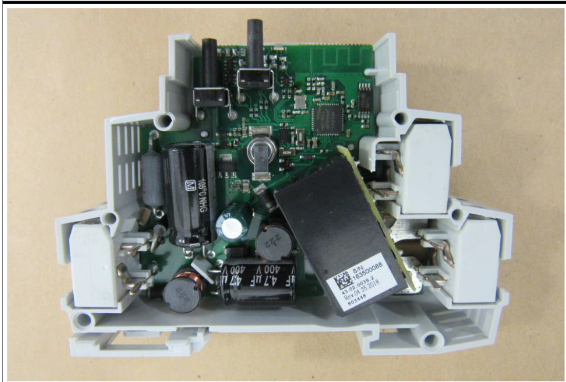
EUT INTERNAL VIEW (B)
