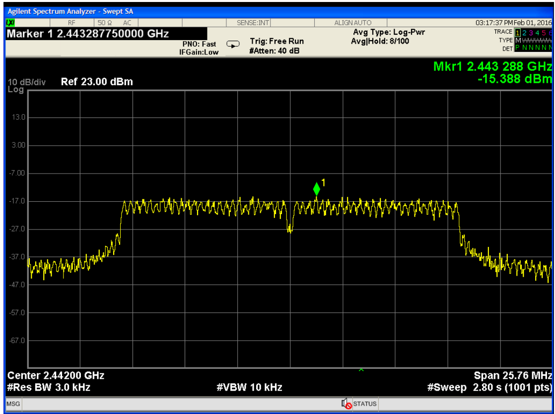
Channel 7:2.442GHz:
