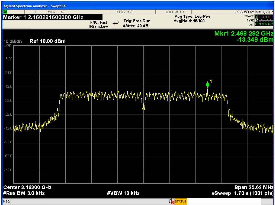
Channel 11:2.462 GHz:
