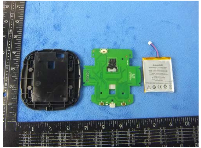
Cover Off - Top View 2(cover with glue)
