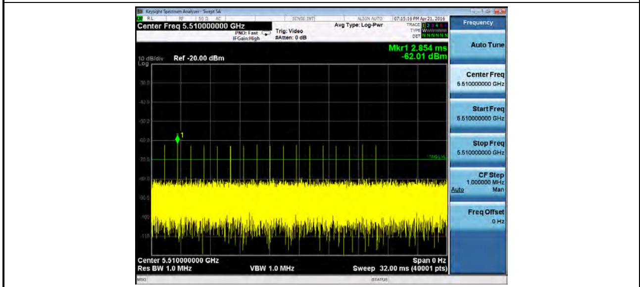
Calibration Radar #0 detection threshold level
