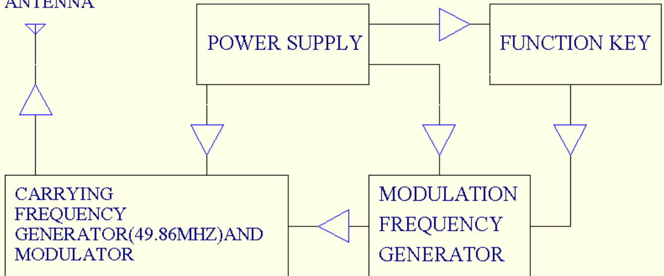
49.86MHZ TX BLOCK DIAGAM
