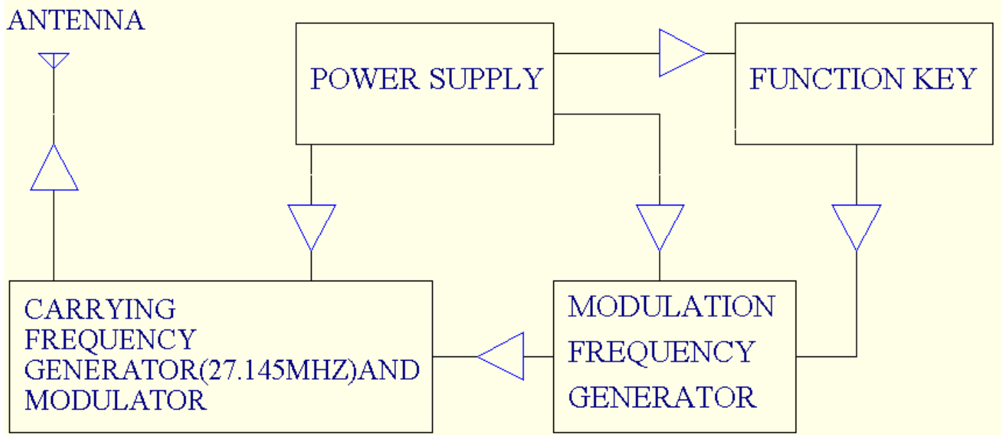
27.145MHZ TX BLOCK DIAGAM
