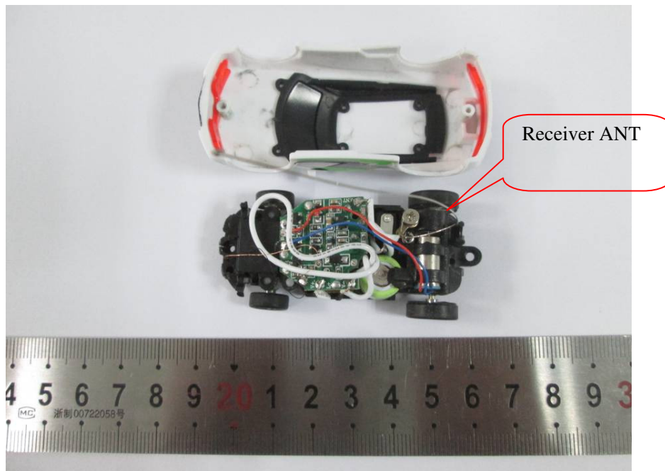
EUT – Cover off View
