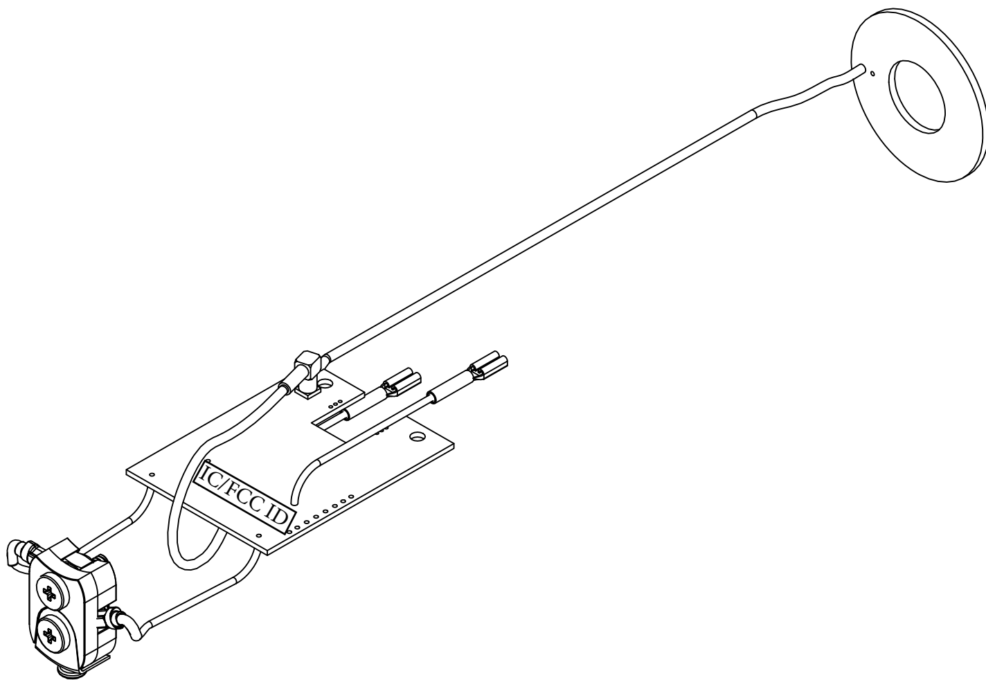
ASSEMBLED VIEW
