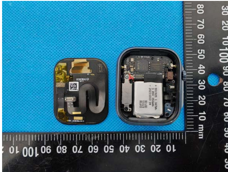
Model: GTX13(equipped with motor 1+speaker 1)
