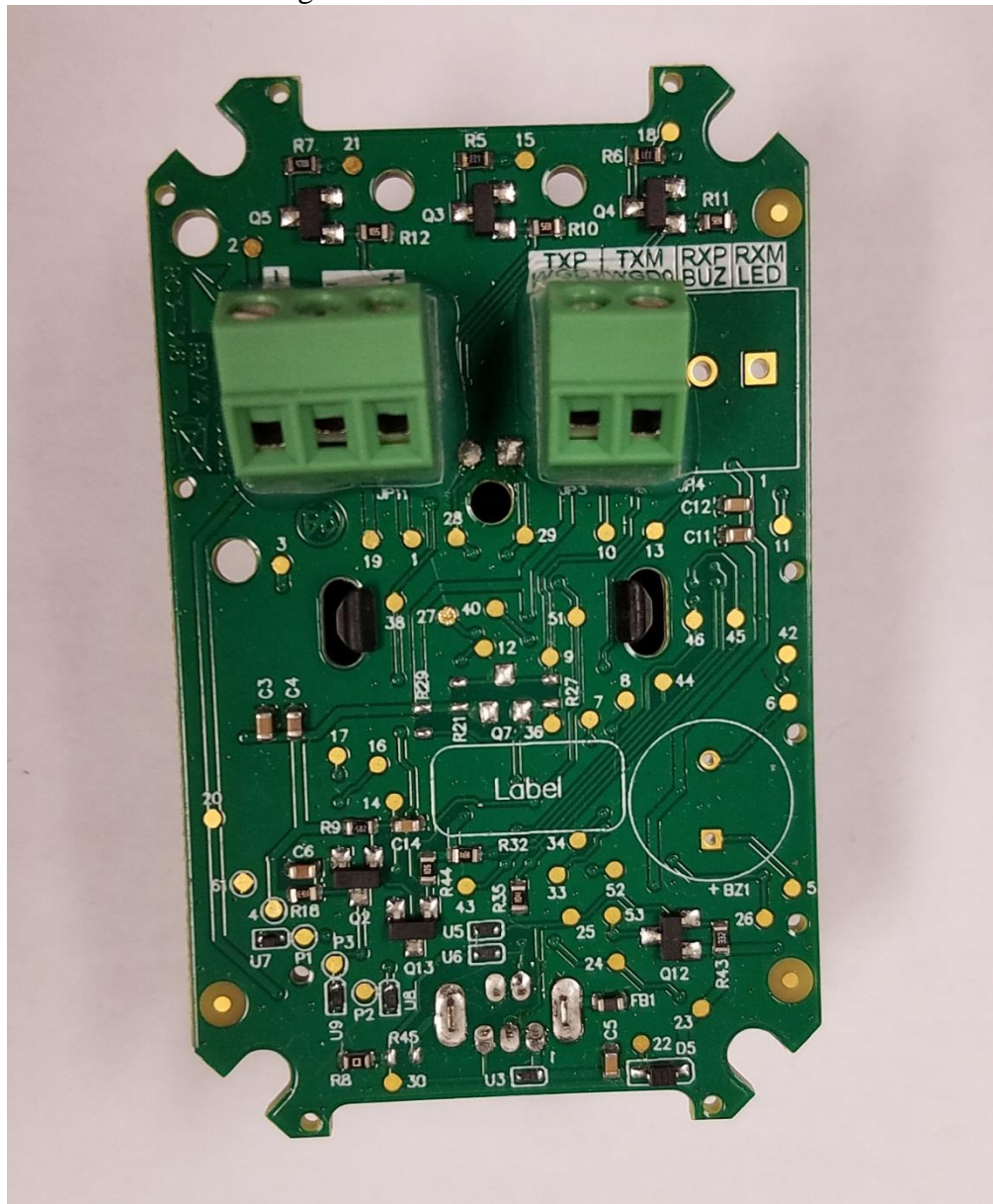
Figure 3 – EUT Internal PCB – back
