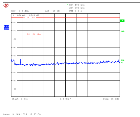
Figure 7.5.1.2-4: 3 GHz – 25 GHz – MCH
