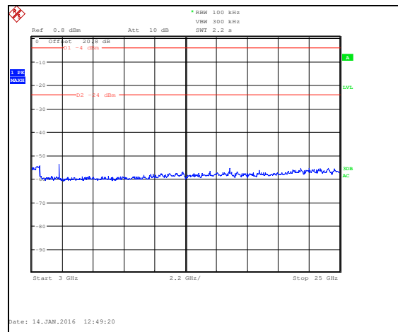
Figure 7.5.1.2-2: 3 GHz - 25 GHz – LCH
