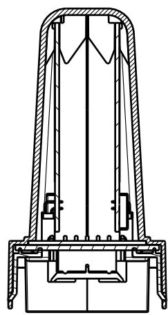
SECTION Z-Z
