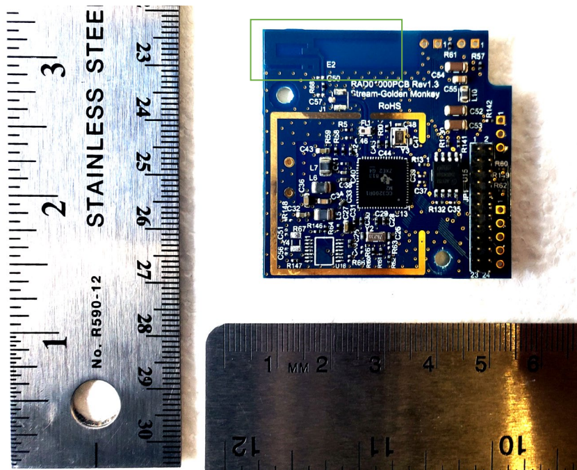
Figure 4. PSB 1 Top
