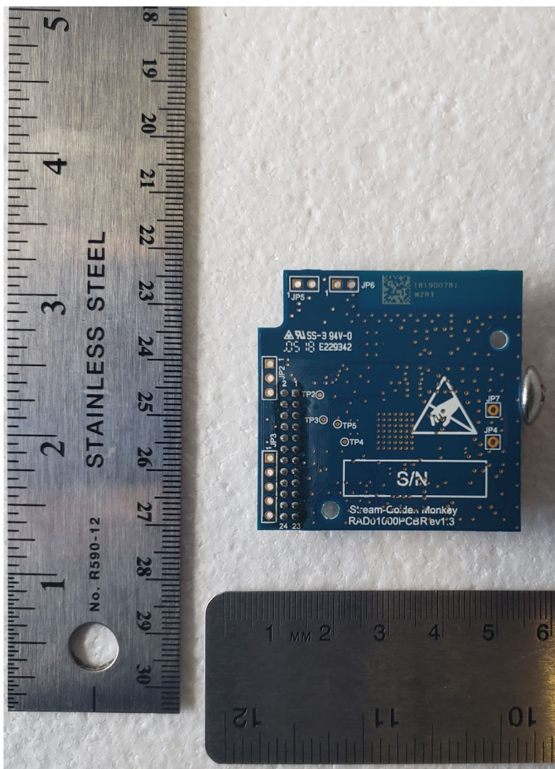
Figure 5. PSB 1 Bottom
