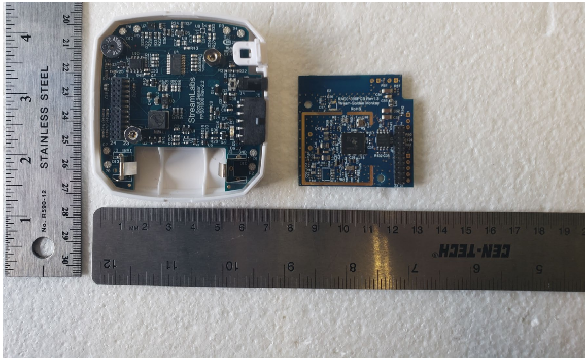
Figure 3. PCB Separated
