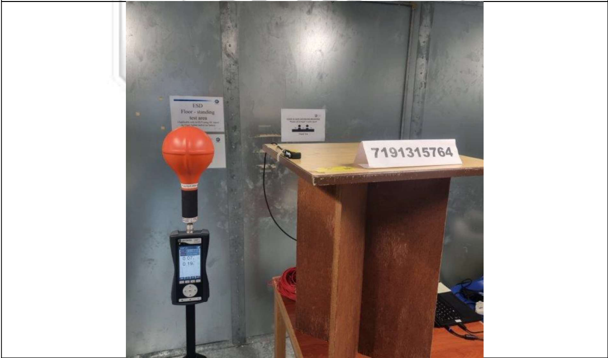
Maximum Permissible Exposure (MPE) Test Setup
