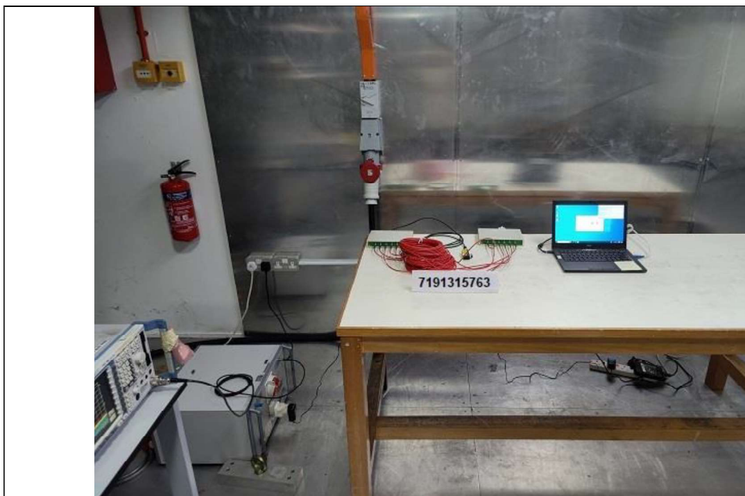
Conducted Emissions Test Setup (Front View)
