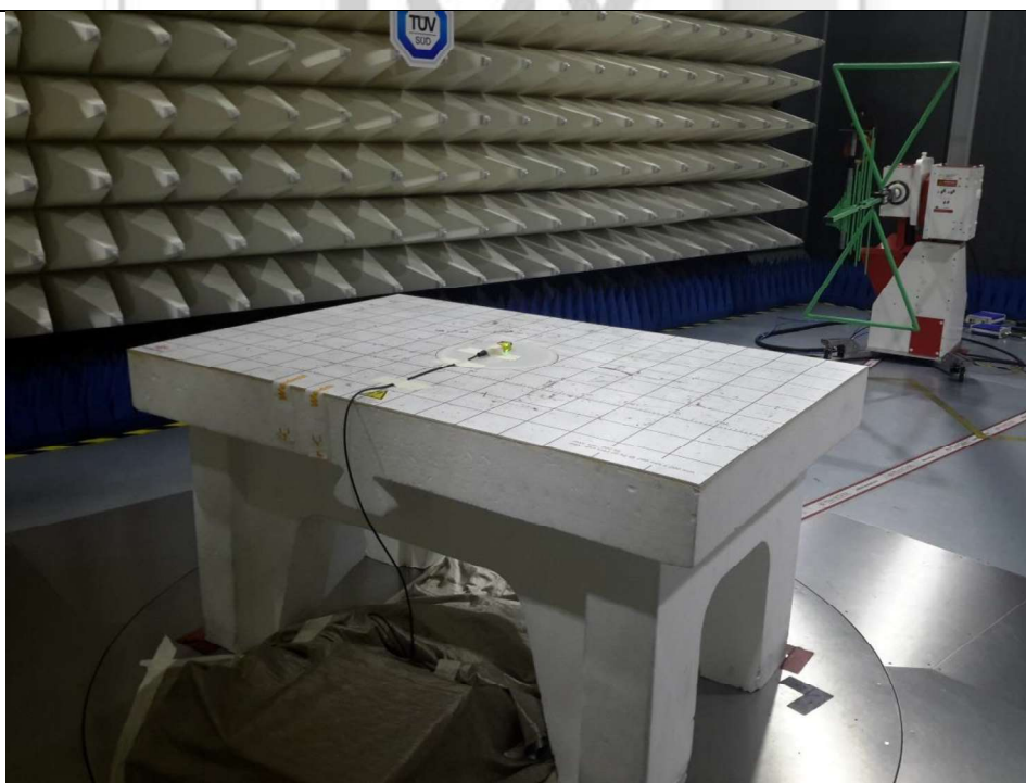
Radiated Emissions (Spurious Emissions Inclusive Restricted Bands Requirement) Test Setup (Rear View)
