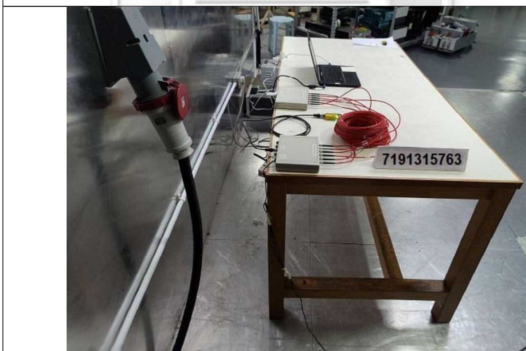
Conducted Emissions Test Setup (Rear View)
