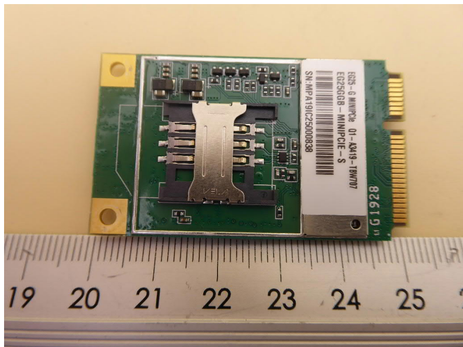
Module PCB, bottom view
