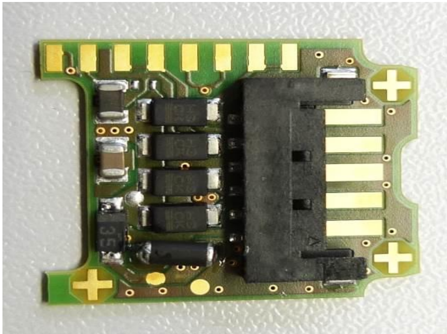
Photo 4: PCB 2 front side view
