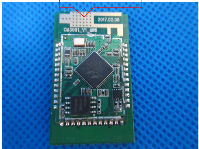
WiFi Antenna
