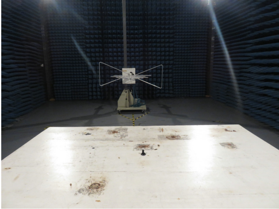
1 Photo of Radiation Emission Test
