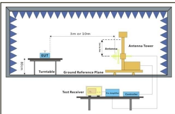
30MHz-1GHz
