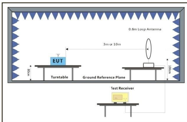
Below 30MHz
