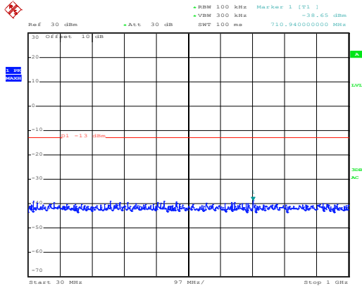
30MHz~1GHz
