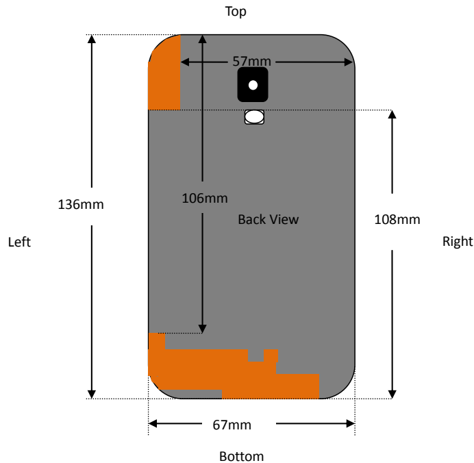
Fig.14.1 EUT Antenna Locations
