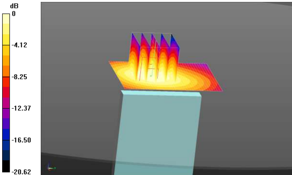
0 dB = 0.537 W/kg = -2.70 dBW/kg
