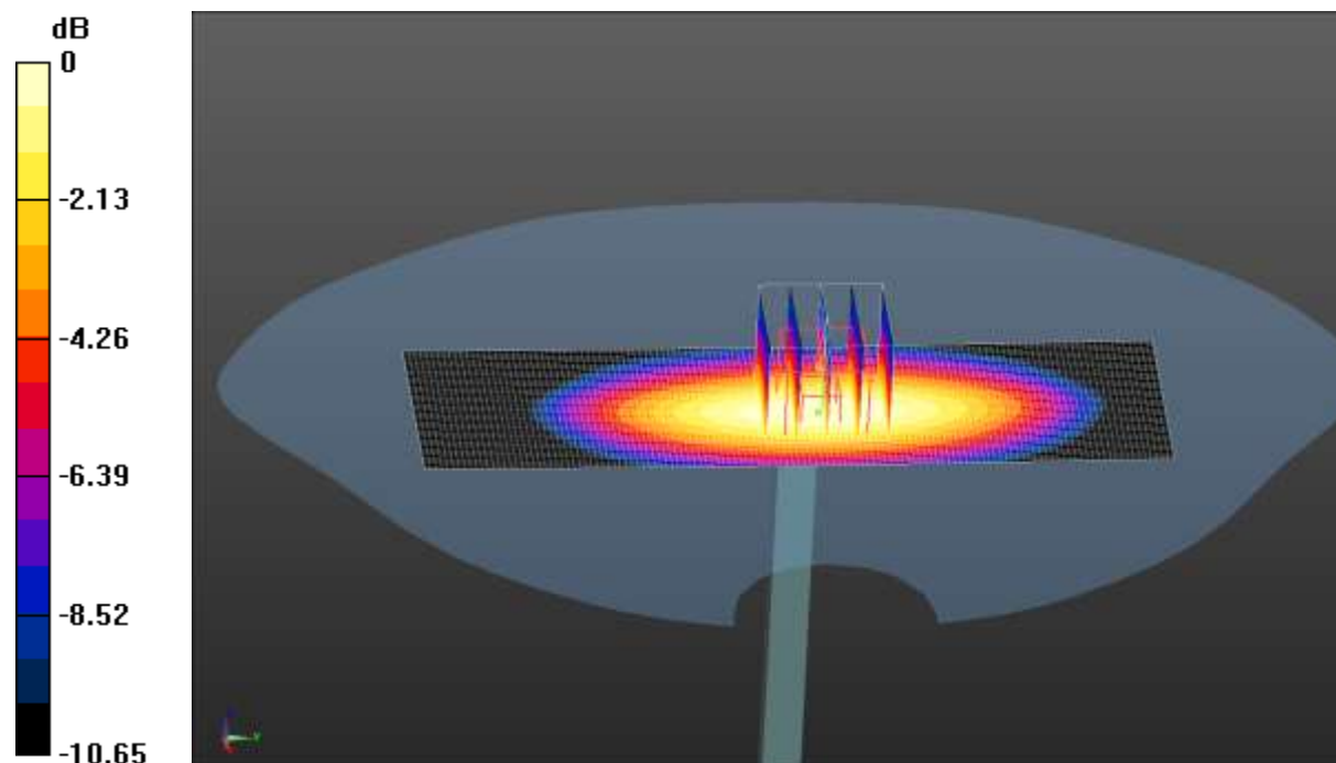
0 dB = 0.504 W/kg = -2.98 dBW/kg
