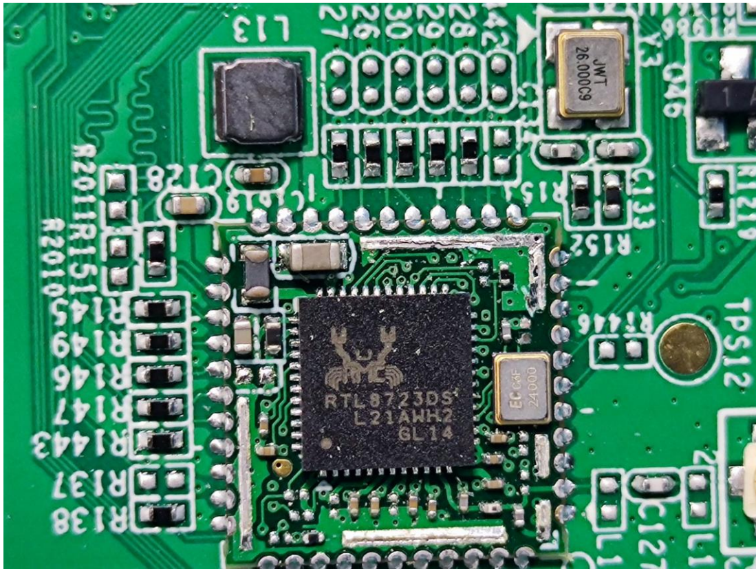
WiFi/Bluetooth Module
