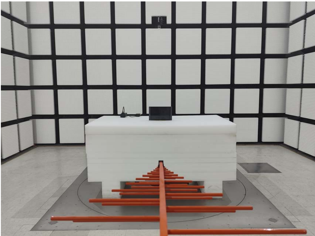
Radiated Emission Below 1GHz View-PoE power mode
