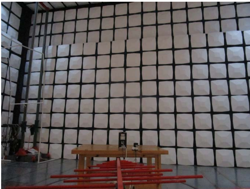
Radiated Emission- Rear View (Adapter Power Supply)
