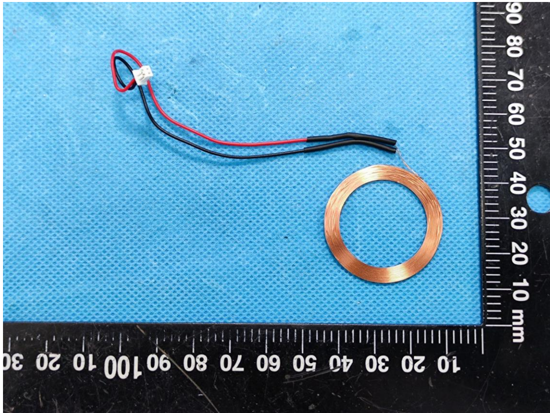
125kHz Antenna
