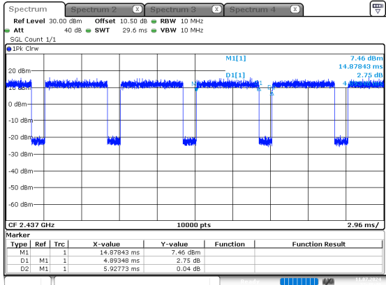
n40_2437MHz_Chain 0
