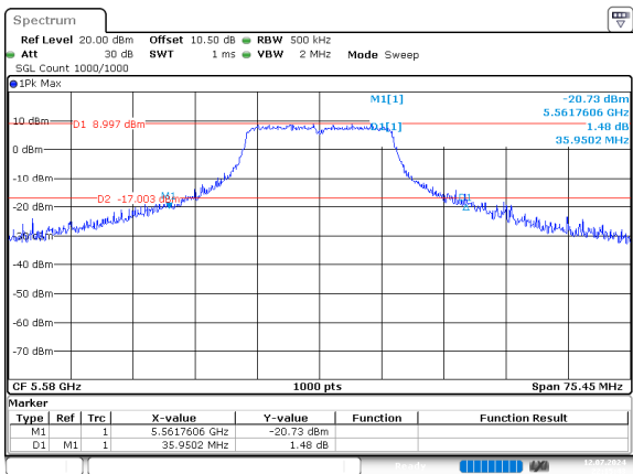
n20_5580MHz_Chain 0
