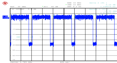
a_5785MHz_Chain 0
