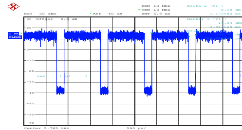
n20_5785MHz_Chain 0
