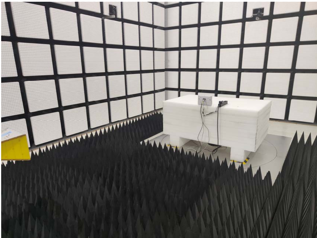
Radiated Emission Above 1G rear View-AC/DC Adapter
