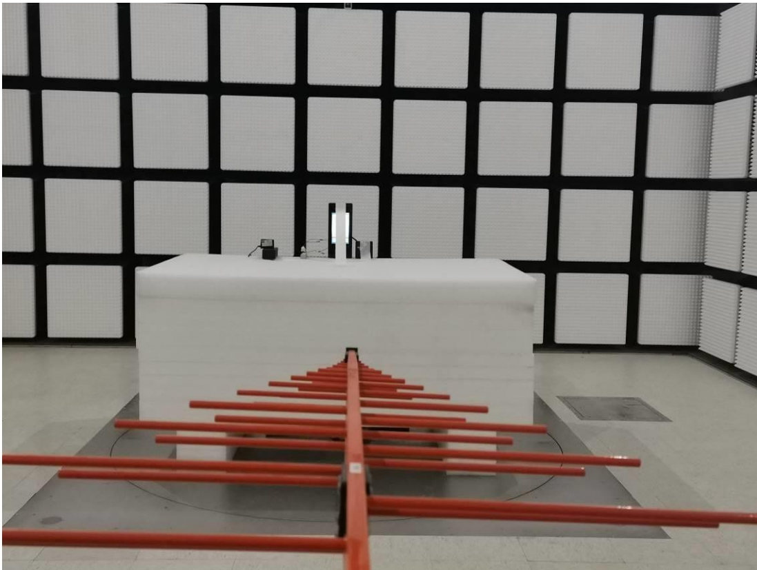
Radiated Emission Below 1G rear View Adapter
