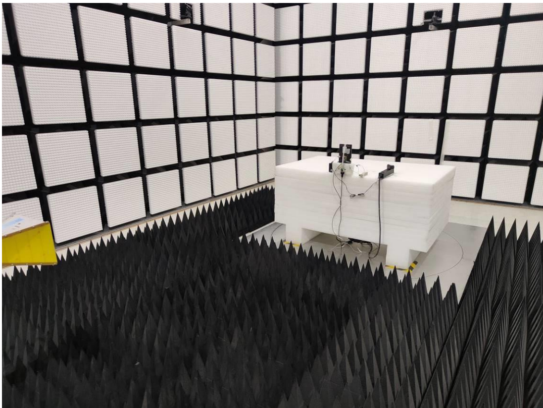
Radiated Emission Above 1G rear View Adapter
