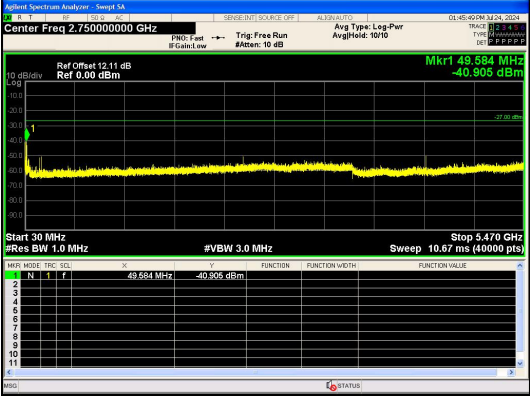
Spurious Emission:30.0~5470 MHz IEEE 802.11n_Channel 100_20MHz_Antenna 0
