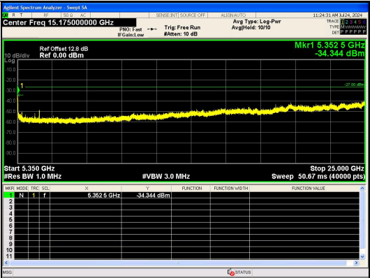
Spurious Emission:5350~25000.0 MHz IEEE 802.11n_Channel 56_20MHz_Antenna 0
