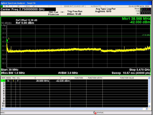
Spurious Emission:30.0~5470 MHz IEEE 802.11n Channel 120_20MHz_Antenna 0
