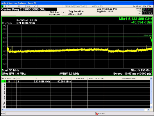
Spurious Emission:30.0~5150 MHz IEEE 802.11n_Channel 56_20MHz_Antenna 0
