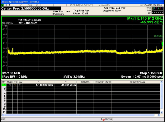
Spurious Emission:30.0~5150 MHz IEEE 802.11n_Channel 52_20MHz_Antenna 0
