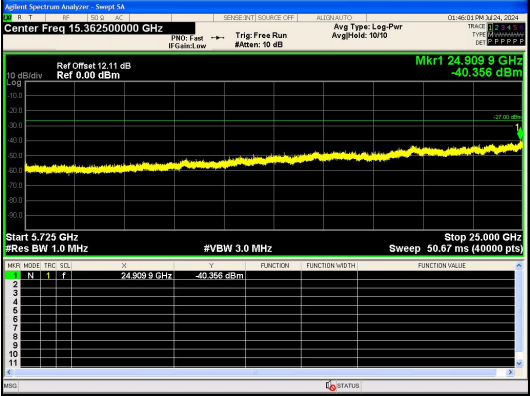
Spurious Emission:5725~25000.0 MHz IEEE 802.11n_Channel 100_20MHz_Antenna 0
