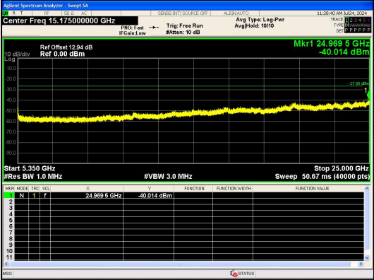
Spurious Emission:5350~25000.0 MHz IEEE 802.11n_Channel 64_20MHz_Antenna 0
