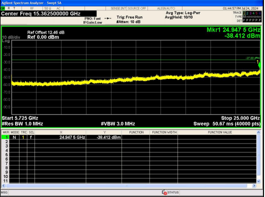
Spurious Emission:5725~25000.0 MHz IEEE 802.11n Channel 140_20MHz_Antenna 0
