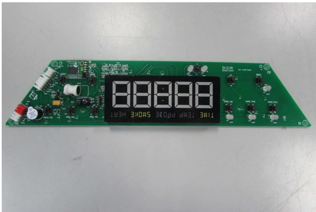
Control circuit PCB view
