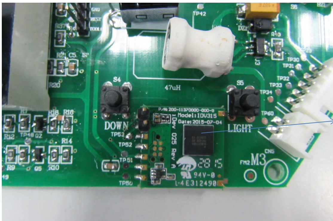
Bluetooth module View
