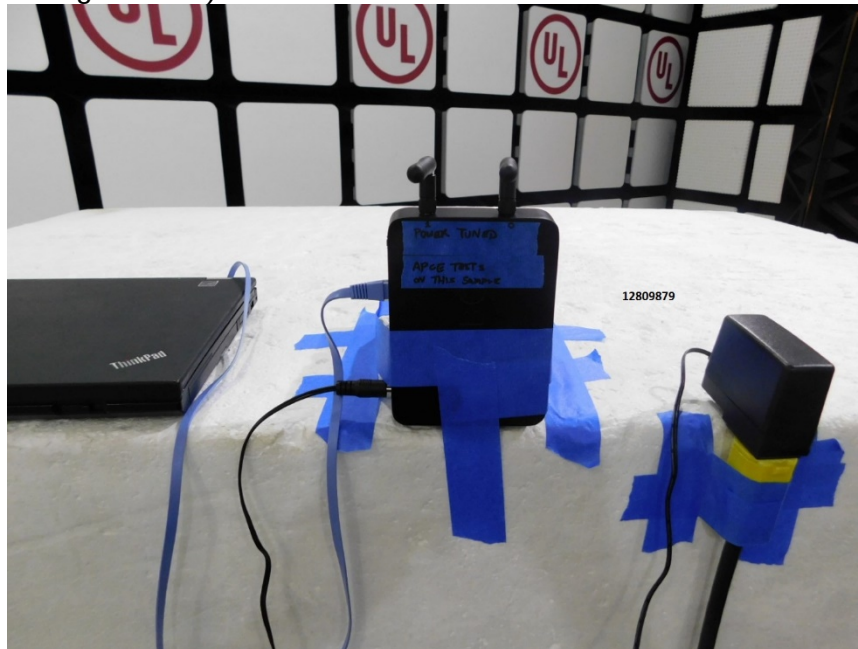
RADIATED SPURIOUS PHOTO (Z Orientation, Antenna Configuration 1)
