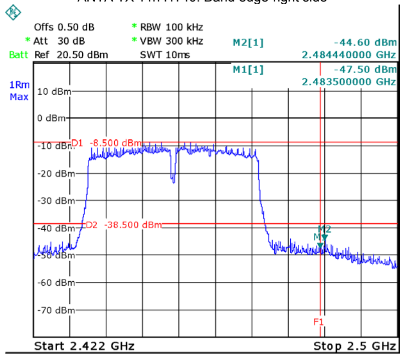
ANTA TX 11n HT40: Band edge-right side
