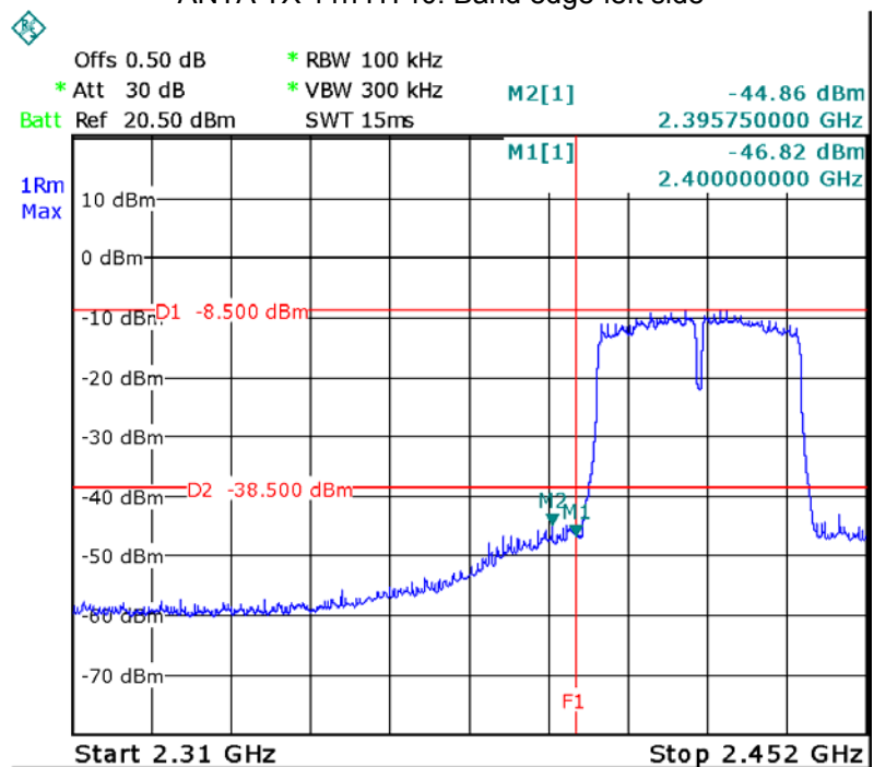
ANTA TX 11n HT40: Band edge-left side
