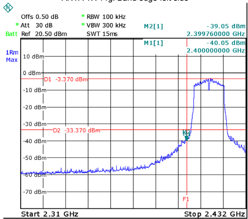
ANTA TX 11g: Band edge-left side
