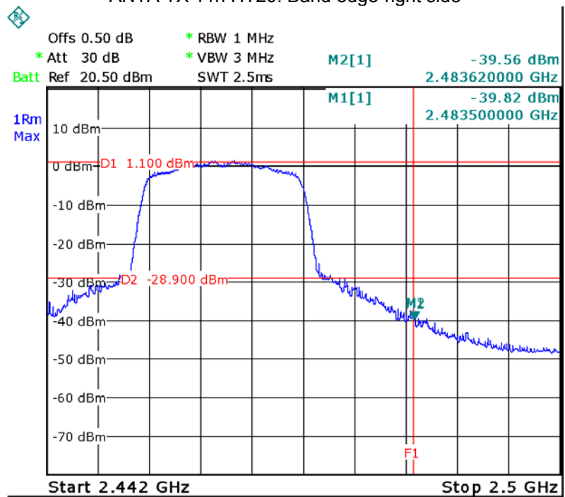
ANTA TX 11n HT20: Band edge-right side
