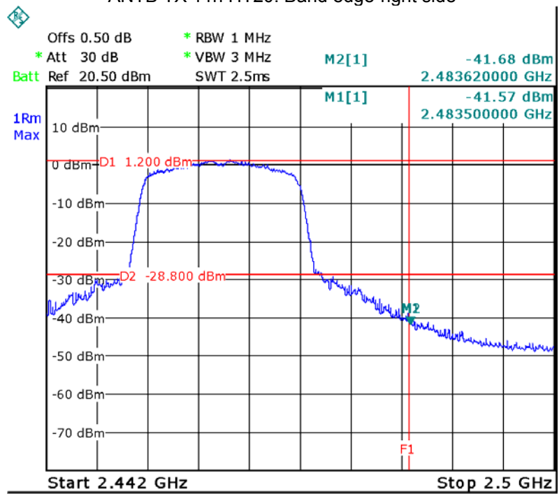
ANTB TX 11n HT20: Band edge-right side
