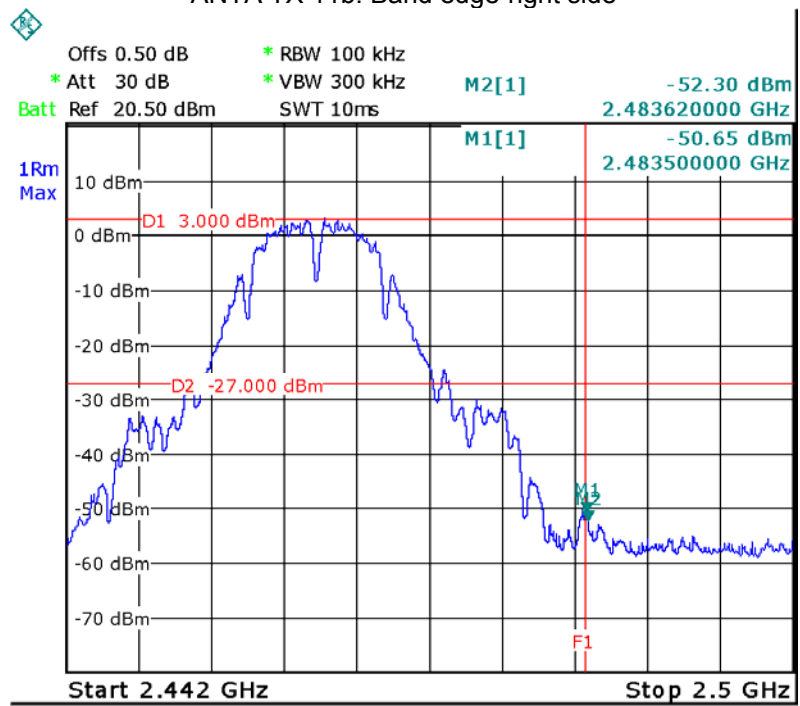
ANTA TX 11b: Band edge-right side
