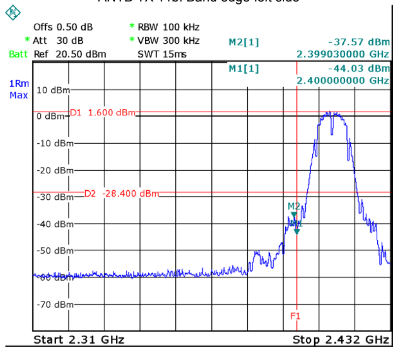
ANTB TX 11b: Band edge-left side
