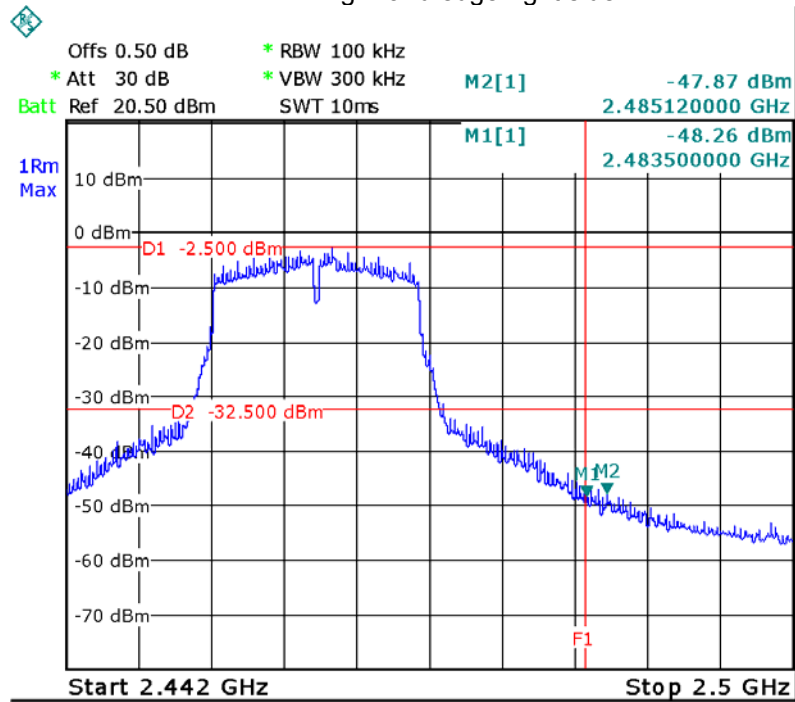
ANTA TX 11g: Band edge-right side
