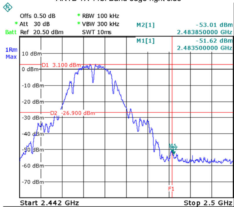
ANTB TX 11b: Band edge-right side
