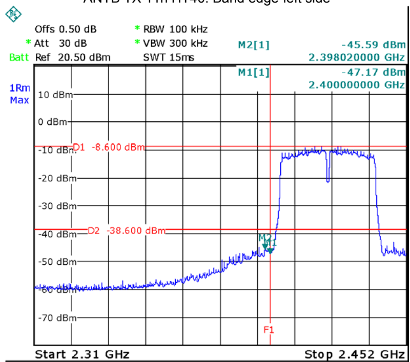
ANTB TX 11n HT40: Band edge-left side
