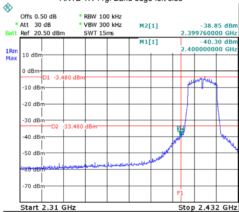
ANTB TX 11g: Band edge-left side
