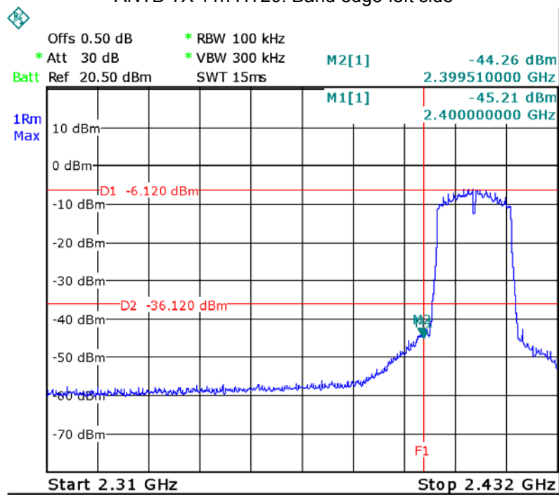
ANTB TX 11n HT20: Band edge-left side
