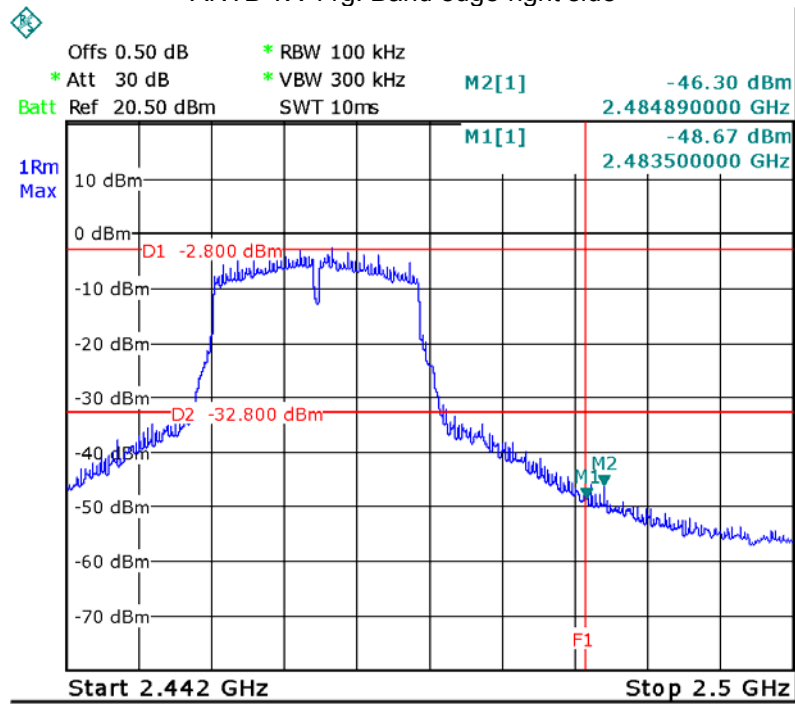
ANTB TX 11g: Band edge-right side
