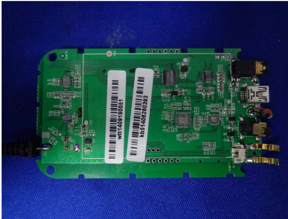
EUT Photo #14- Inside View
